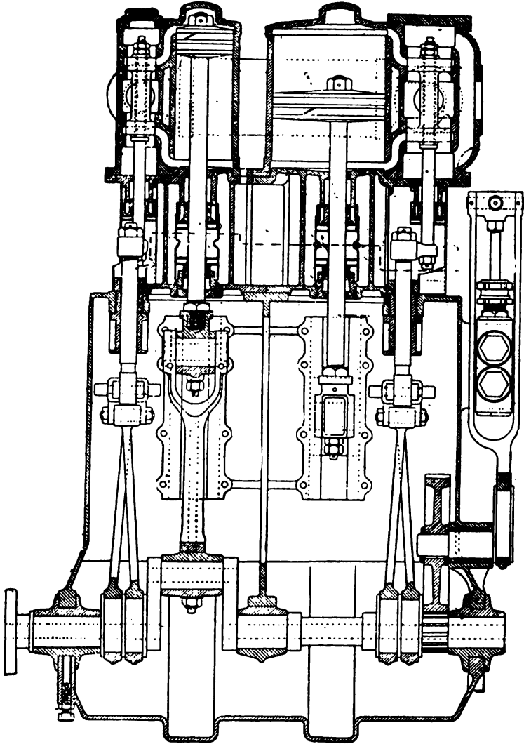
FIG. 277.—The "Lifu" Compound Steam Engine for heavy vehicle use. This section is drawn through the centre of the cylindrical steam chests, which, as in the Thornycroft engine (Fig. 273), are below and at the sides of the steam cylinders. The appearance of eccentricity in the attachment of the piston rods may thus be understood.
